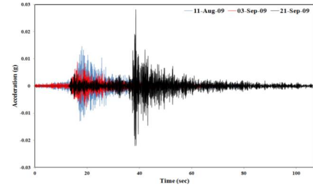
Fig.3: Acceleration time history of input motions
