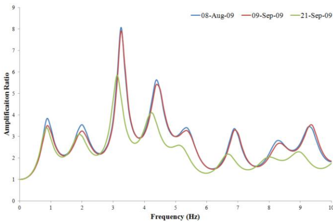
Fig. 15: Amplification Spectrum
